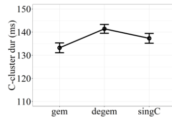
Figure 3: Total C-cluster durations obtained from the acoustic signal
