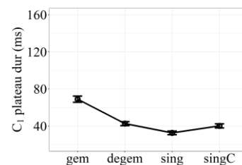
Figure 4: C_1 plateau duration obtained from the articulatory signals
